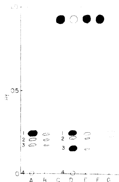
Figure 1. Representation of the autoradiograms of metabolites from 2,5,2'-trichlorobiphenyl- ^{14}\text{C} and 2,4,5,2',5'-pentachlorobiphenyl- ^{14}\text{C} as separated on a silica gel HF thin-layer chromatogram (TLC). The TLC plate was developed by using n -hexane-ethanol-acetic acid (10:2:1). Metabolic products were arbitrarily designated as M-1, -2, -3, and -4 according to the position on the chromatogram (also see Table I): (A) 2,5,2'-trichlorobiphenyl- ^{14}\text{C} supernatant extract; (B) 2,5,2'-trichlorobiphenyl- ^{14}\text{C} cell extract; (C) 2,5,2'-trichlorobiphenyl- ^{14}\text{C} ; (D) 2,4,5,2',5'-pentachlorobiphenyl- ^{14}\text{C} supernatant extract; (E) 2,4,5,2',5'-pentachlorobiphenyl- ^{14}\text{C} cell extract; (F) 2,4,5,2',5'-pentachlorobiphenyl- ^{14}\text{C} ; (G) 2-chlorobenzoic acid (detected under uv light).
